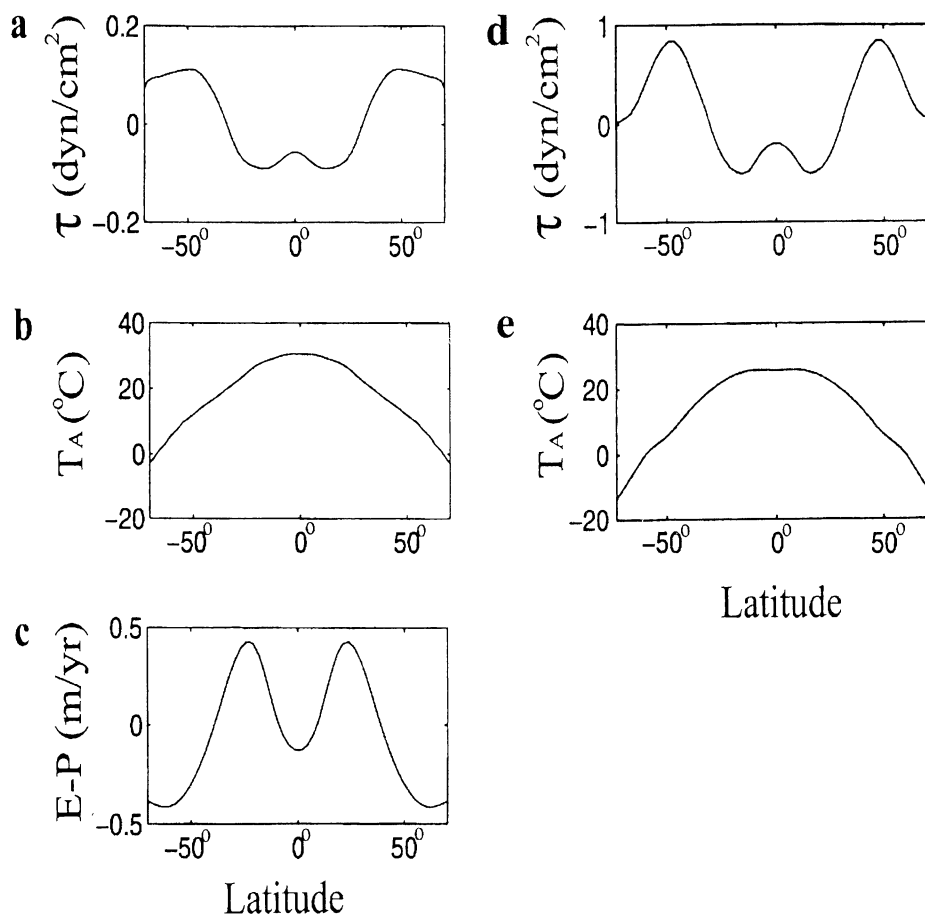
Figure 5. Surface forcing scenario 1 (Figures 5a-5c) and surface forcing scenario 2 (Figures 5d and 5e). (a) Zonally averaged surface wind stress ( \text{dyn}/\text{cm}^2 ). (b) Zonally averaged prescribed surface temperature T_A ( ^{\circ}\text{C} ). (c) Zonally averaged freshwater flux ( E - P ) ( \text{m}/\text{yr} ). (d) Zonally averaged surface wind stress ( \text{dyn}/\text{cm}^2 ). (e) Zonally averaged prescribed surface temperature T_A ( ^{\circ}\text{C} ).
